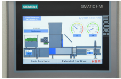
Control of the pressing process via light barrier
