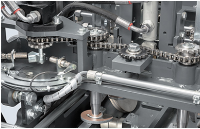
Fully automatic vertical strapping with wire
